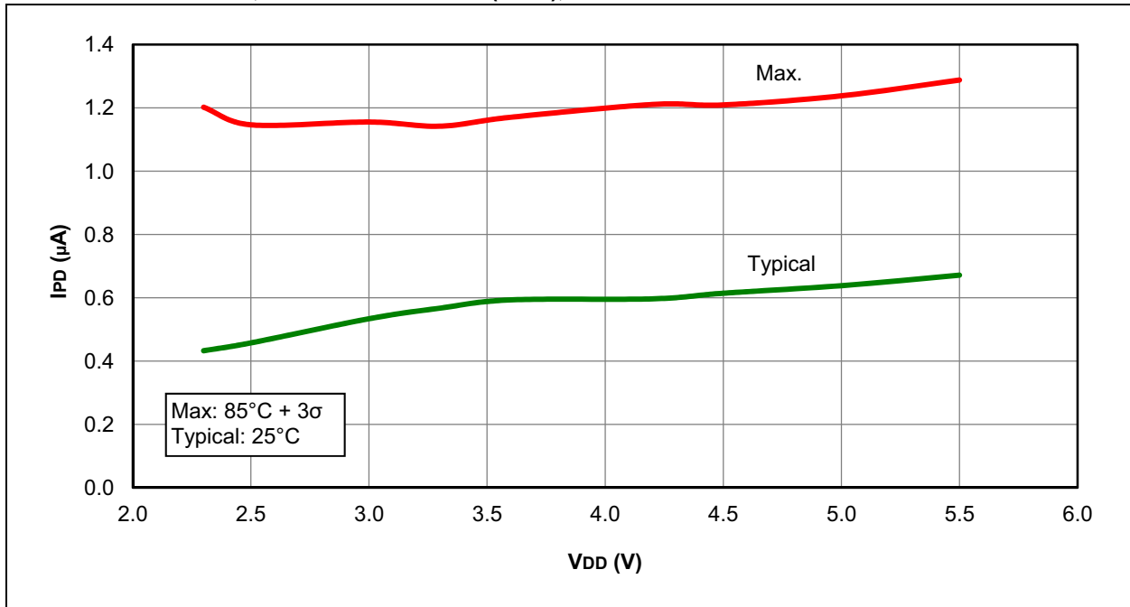
FIGURE 26-24: I PD , WATCHDOG TIMER (WDT), PIC16F1507 ONLY
