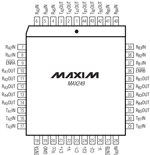
PLCC
