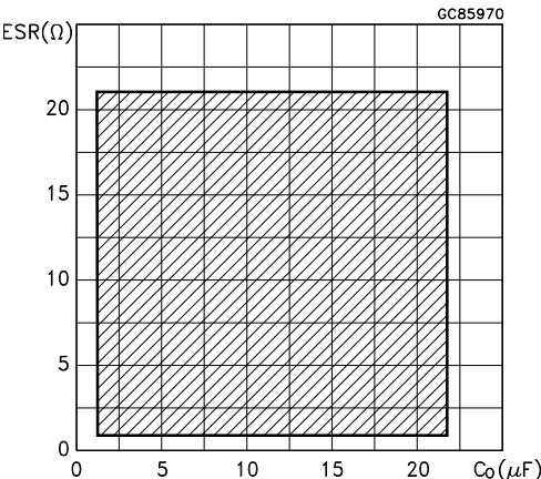
Figure 21. Stability for 2.85 V
