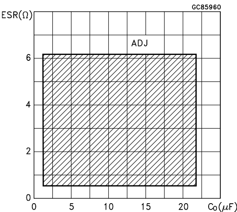
Figure 20. Stability for adjustable
