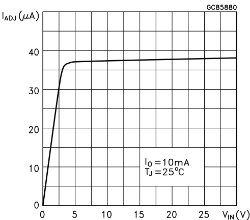
Figure 11. Adjust pin current vs. input voltage
