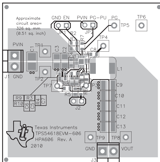
Figure 15. TPS54618EVM-606 Top-Side Assembly
