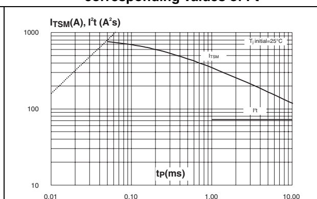
Figure 8. Non-repetitive surge peak on-state current for a sinusoidal pulse with width t_p < 10\text{ms} , and corresponding values of I^2t
