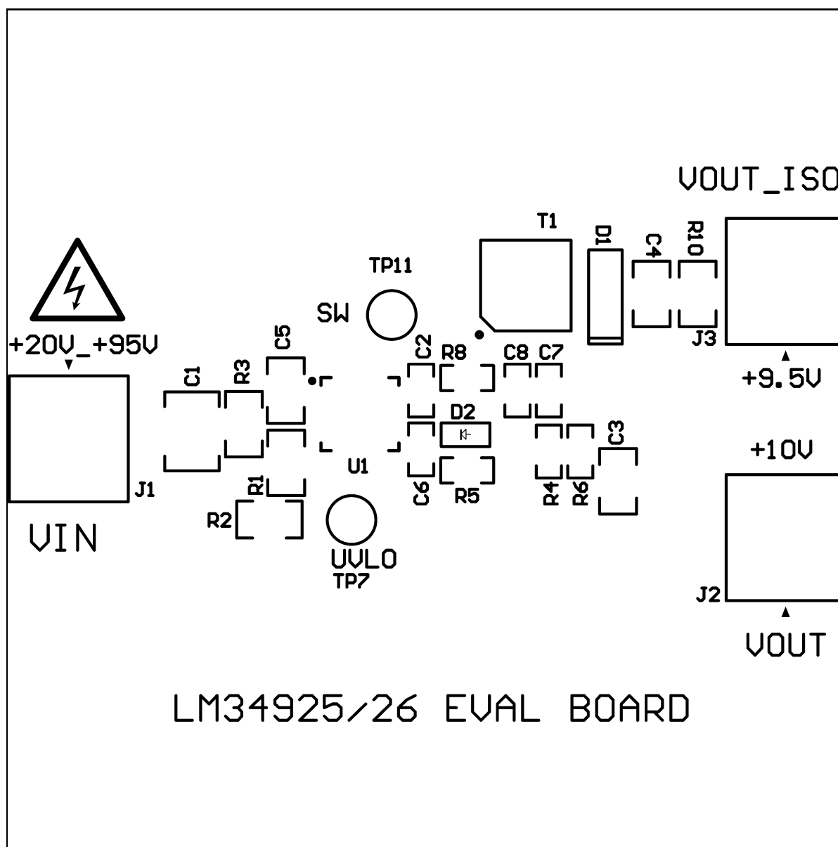
Figure 5. Board Silkscreen
