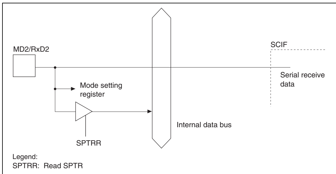
Figure 18.7 MD2/RxD2 Pin
