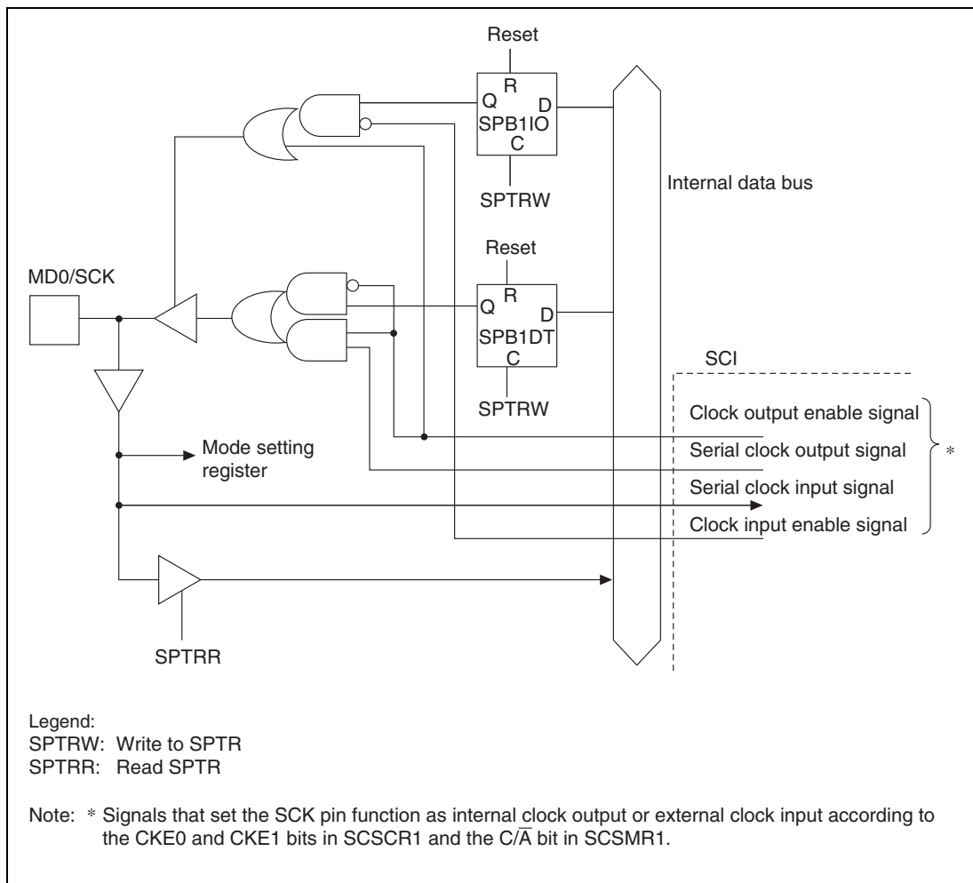
Figure 15.2 MD0/SCK Pin
