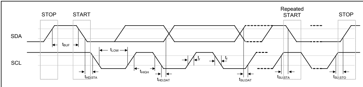
Figure 5-10 I 2 C Bus Timing
