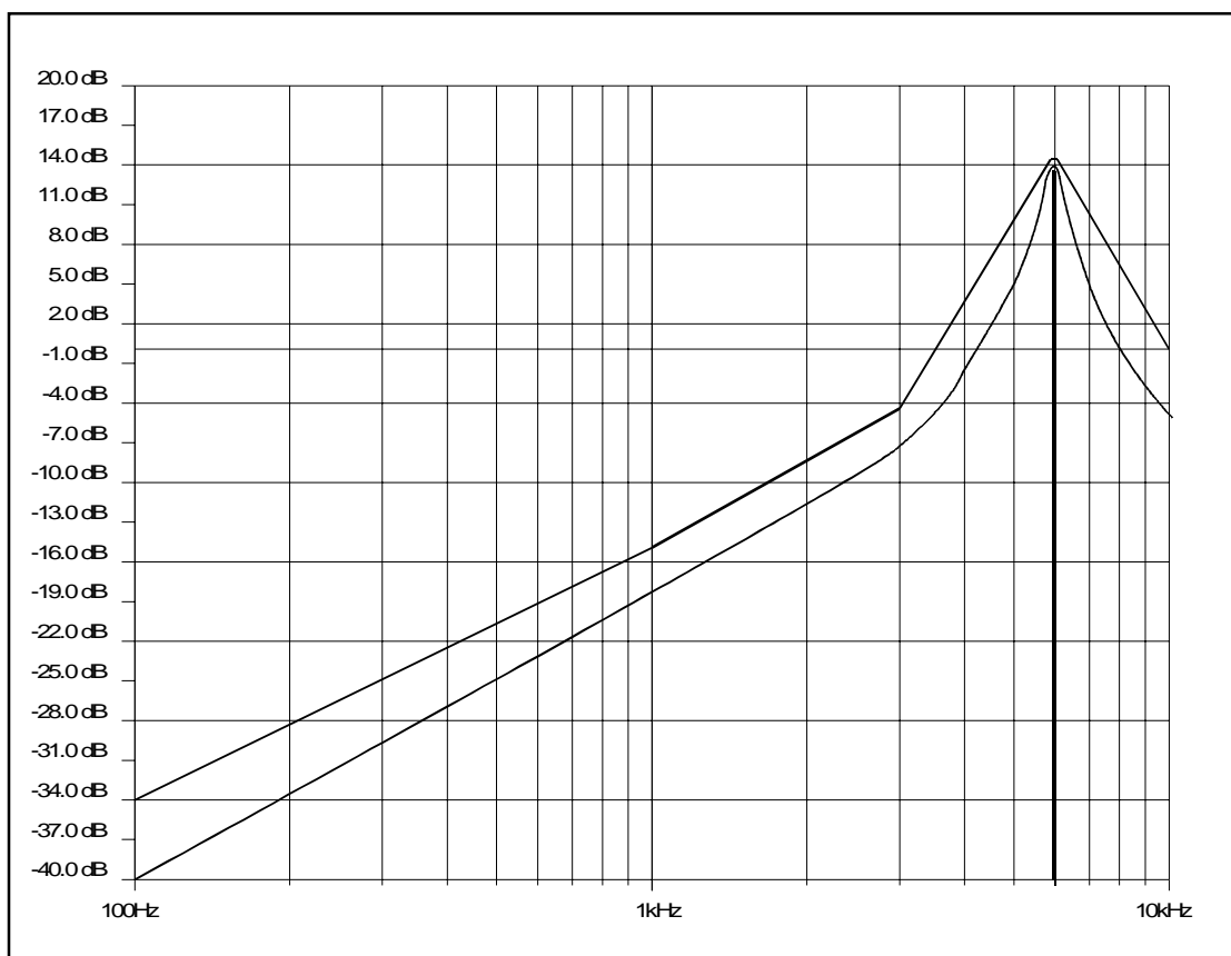
Filter F2 frequency response
