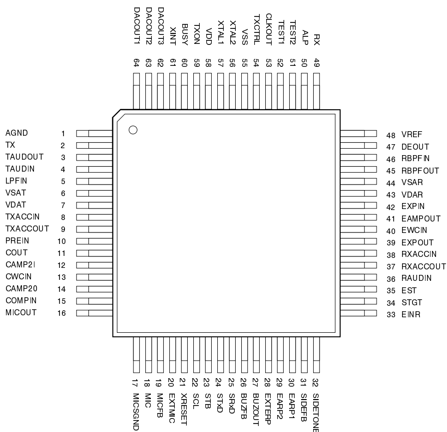
TQFP64 package
