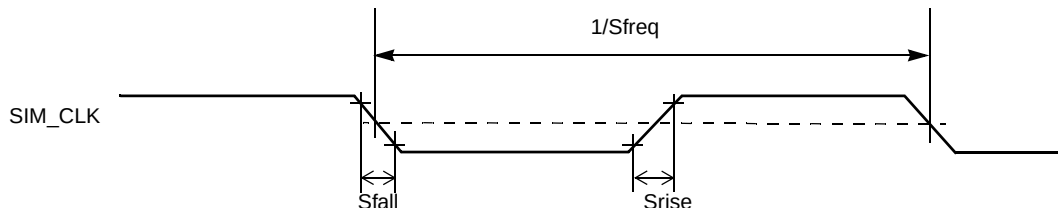
Figure 30. SIM Clock Timing Diagram
