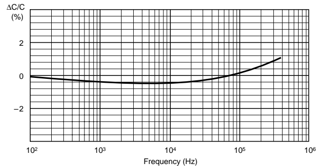
Capacitance change
