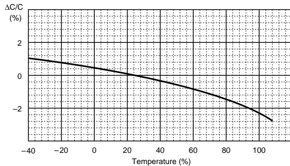
Capacitance change
