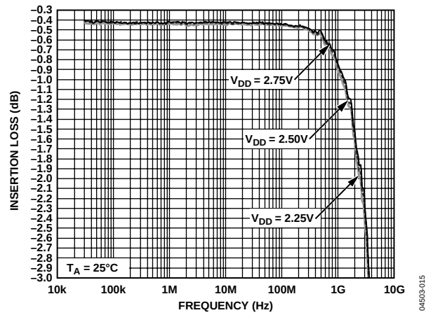
Figure 7. Insertion Loss vs. Frequency over Supplies (S12 and S21)
