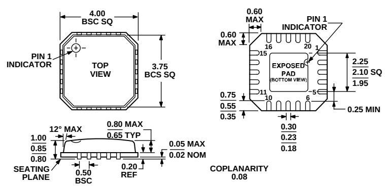
Figure 31. 20-Lead Lead Frame Chip Scale Package [LFCSP_VQ] 4 mm × 4 mm Body, Very Thin Quad (CP-20-1) Dimensions shown in millimeters
