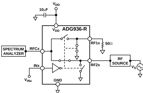
Figure 26. P_{-1dB}
