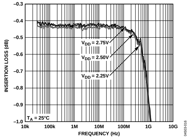
Figure 8. Insertion Loss vs. Frequency over Supplies (S12 and S21) (Zoomed Figure 7)
