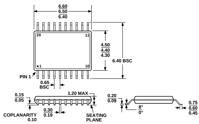
Figure 30. 20-Lead Thin Shrink Small Outline Package [TSSOP] (RU-20) Dimensions shown in millimeters
