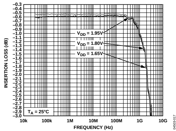
Figure 9. Insertion Loss vs. Frequency over Supplies (S12 and S21)
