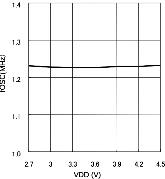
Fig.3 fOSC vs. VDD
