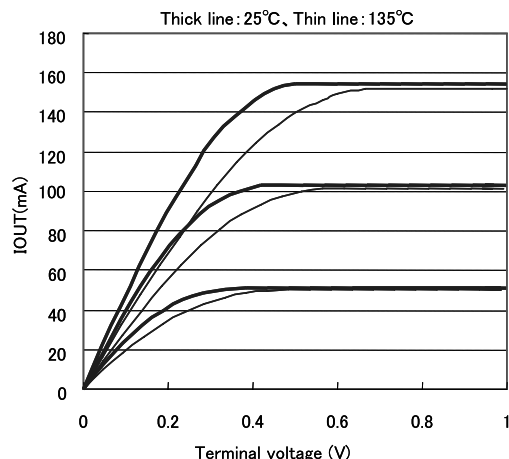
Fig.8 IOUT(B) vs. Terminal voltage
