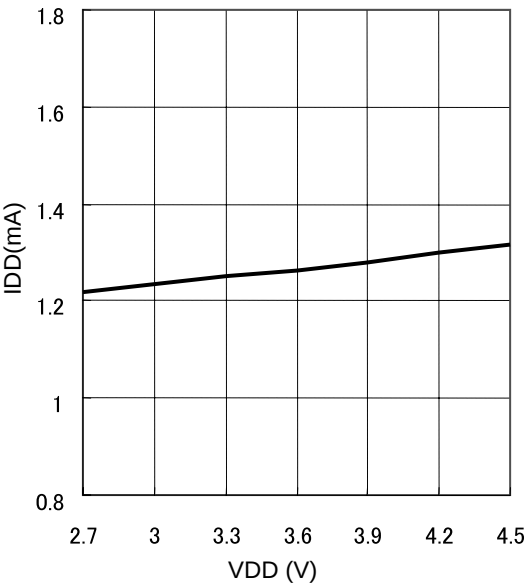
Fig.5 IDD vs. VDD
