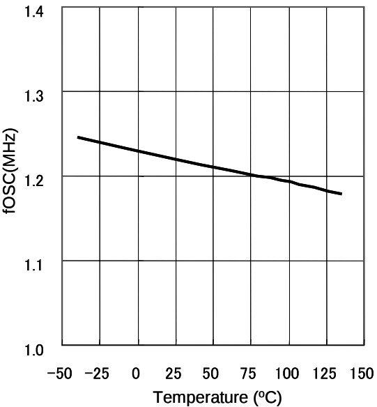
Fig.4 fOSC vs. temperature
