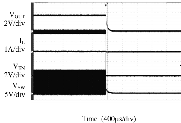
Figure 13. Enable Turn off Characteristic ( I_{\text{OUT}}=2\text{A} , Resistance Load)
