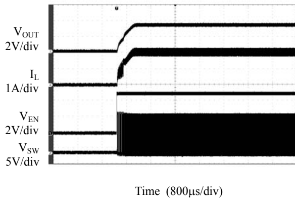
Figure 12. Enable Turn on Characteristic ( I_{\text{OUT}}=2\text{A} , Resistance Load)
