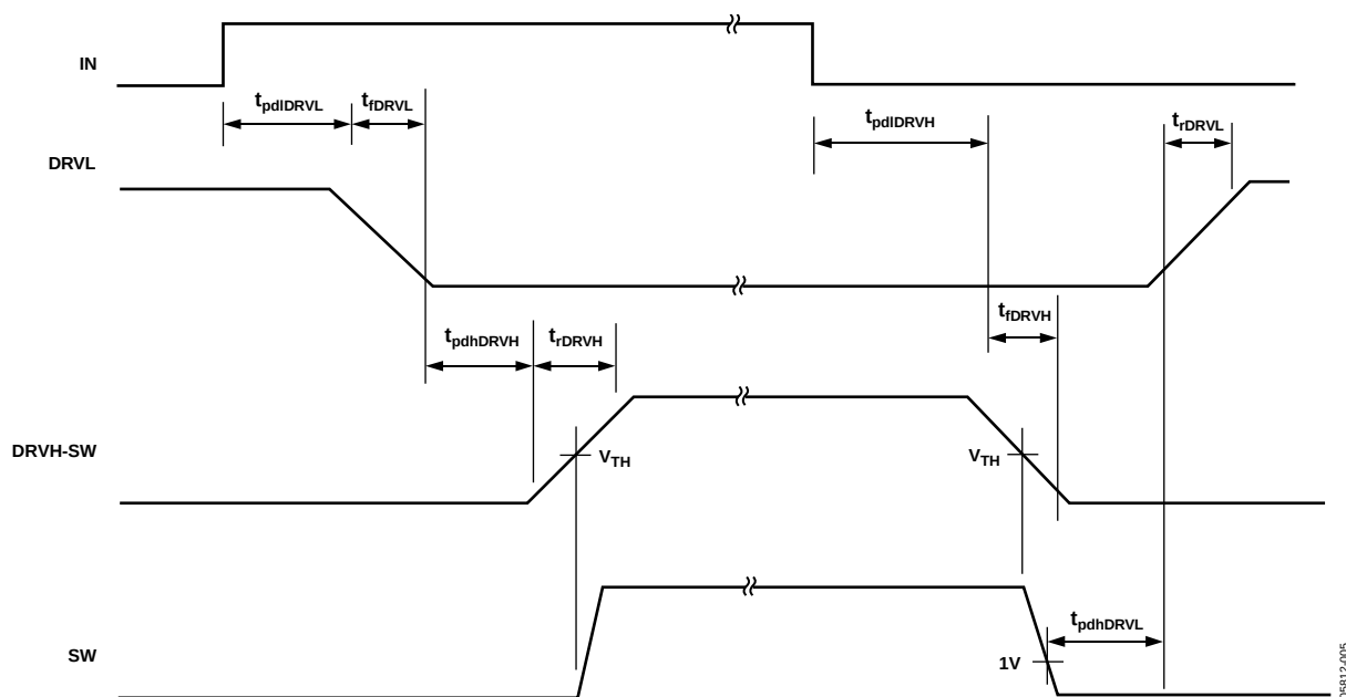
Figure 5. Timing Diagram
