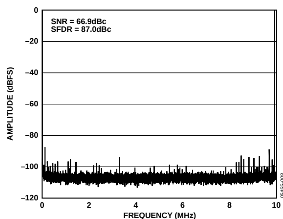
Figure 8. AD9237-20 10 MHz FFT
