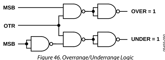
Figure 46. Overrange/Underrange Logic
