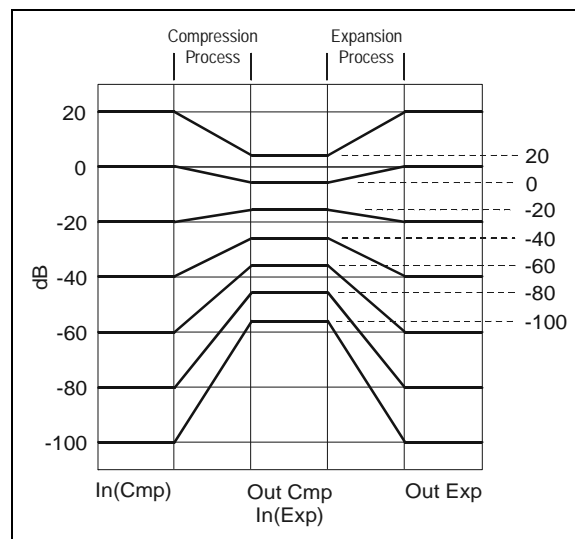
Figure 22. Hi-fi compander transfer characteristics
