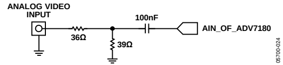
Figure 29. Input Voltage Divider Network
