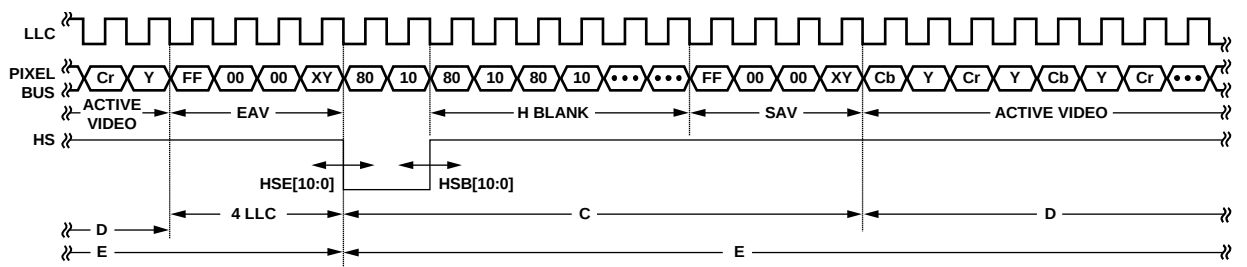
Figure 37. HS Timing
