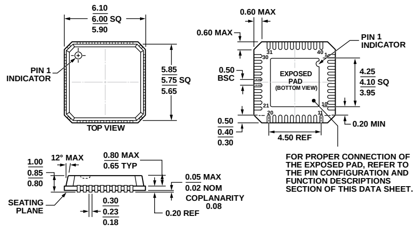
Figure 62. 40-Lead Lead Frame Chip Scale Package [LFCSP_VQ] 6 mm × 6 mm Body, Very Thin Quad (CP-40-1) Dimensions shown in millimeters
