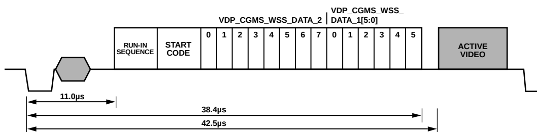
Figure 48. WSS Waveform
