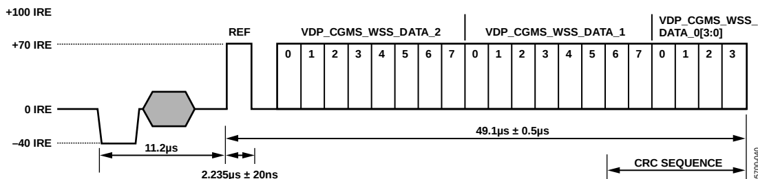
Figure 49. CGMS Waveform
