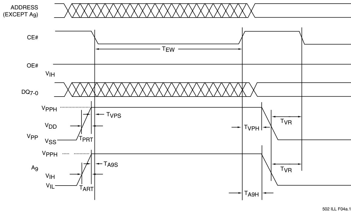
FIGURE 5: CHIP-ERASE TIMING DIAGRAM FOR SST27SF256
