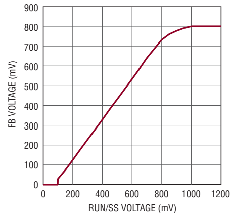
RUN/SS vs FB Voltage
