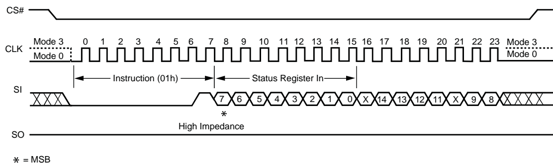
Figure 7.5 Write Status Register Instruction Sequence Diagram
