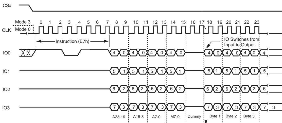
Figure 7.14 Word Read Quad I/O Instruction Sequence (Initial instruction or previous M5-4 ≠ 10)
