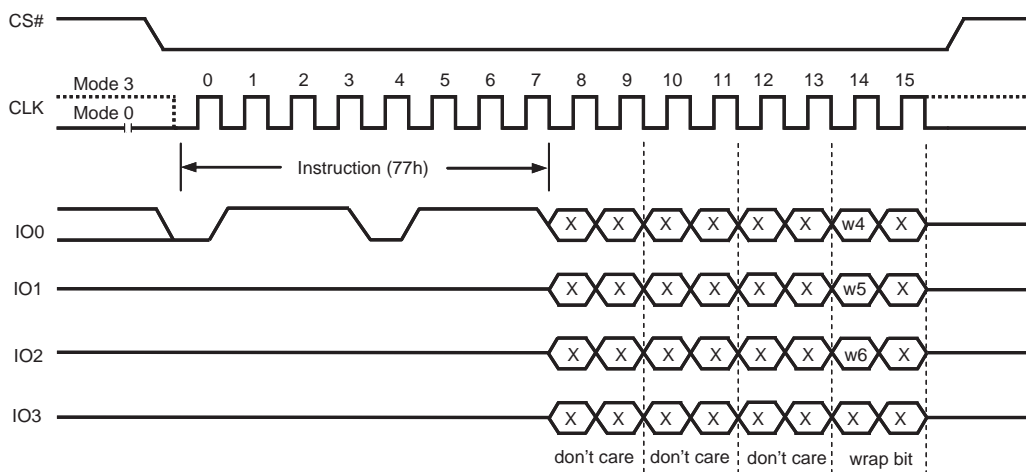
Figure 7.18 Set Burst with Wrap Instruction Sequence
