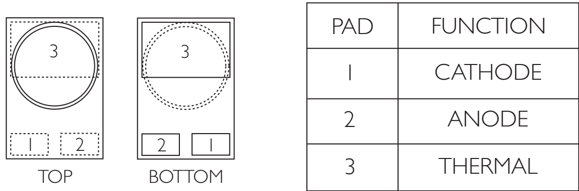
Figure 2. Pad configuration.
