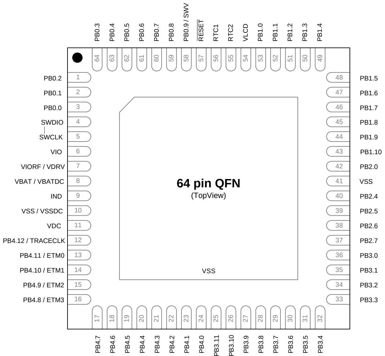
Figure 6.4. SiM3L1x6-GM Pinout
