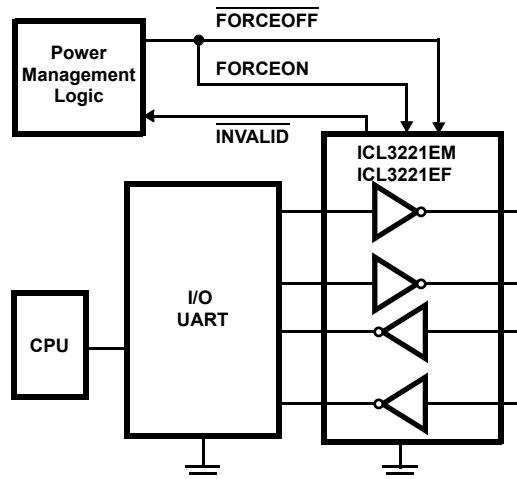
Figure 8. Connections for Manual Powerdown when No Valid Receiver Signals are Present
