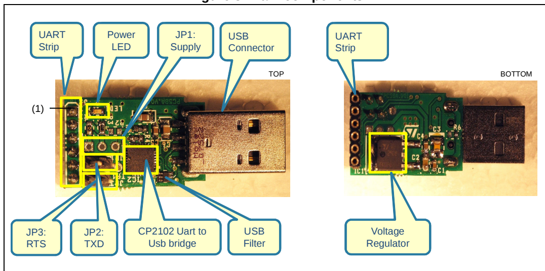
Figure 3. Main components
