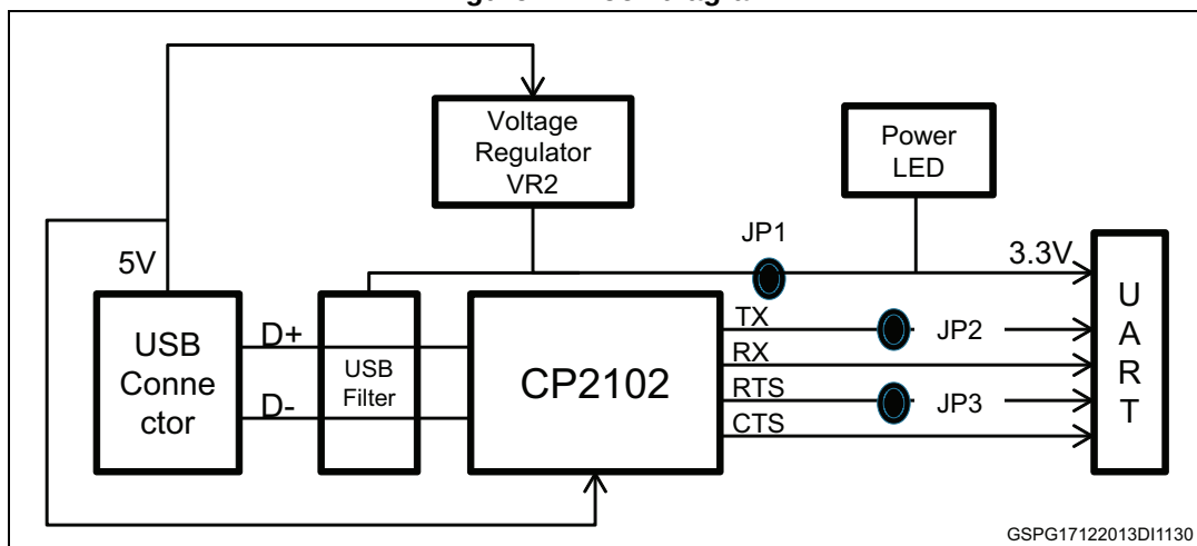
Figure 2. Block diagram
