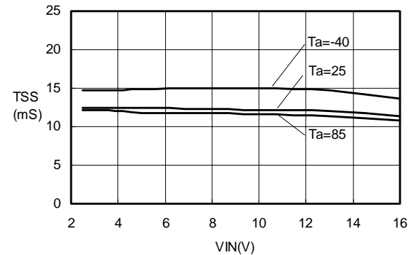
TSS-VIN S-8520/21(Fosc:60kHz)
