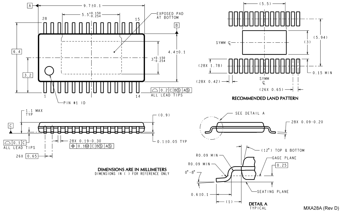
Exposed-DAP TSSOP Package Order Number LM4838MTE NS Package Number MXA28A for Exposed-DAP TSSOP
