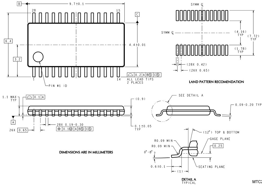
TSSOP Package Order Number LM4838MT NS Package Number MTC28 for TSSOP
