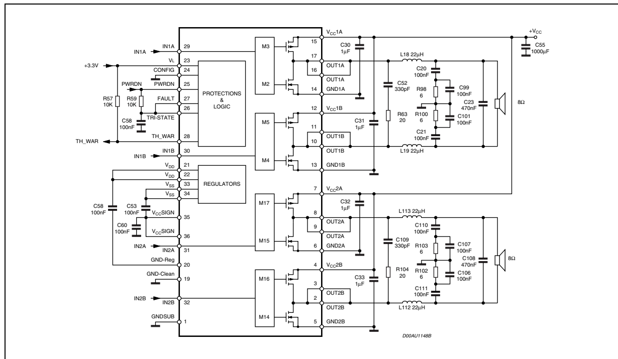
Figure 2. Audio Application Circuit (Dual BTL)
