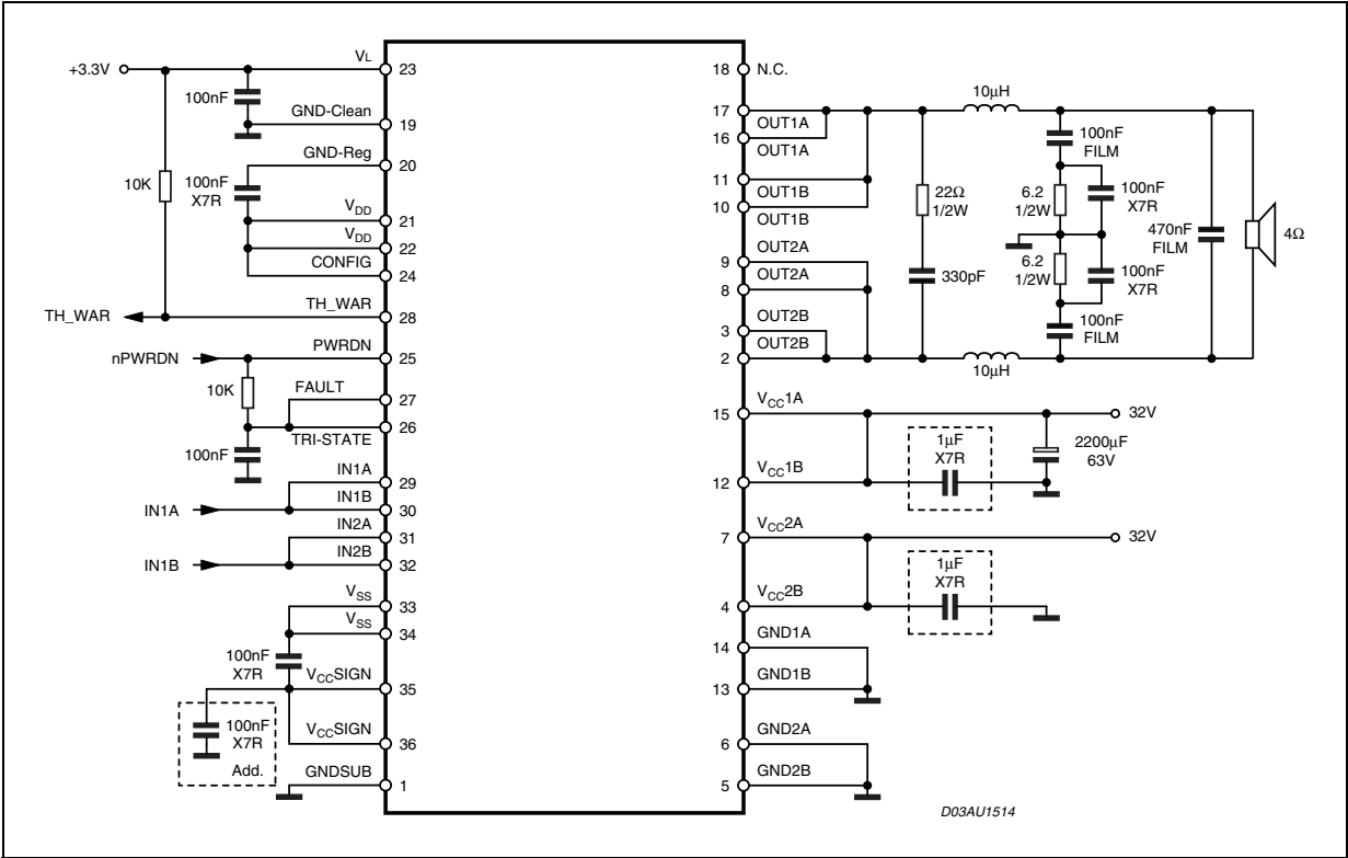
Figure 6. Typical Single BTL Configuration
