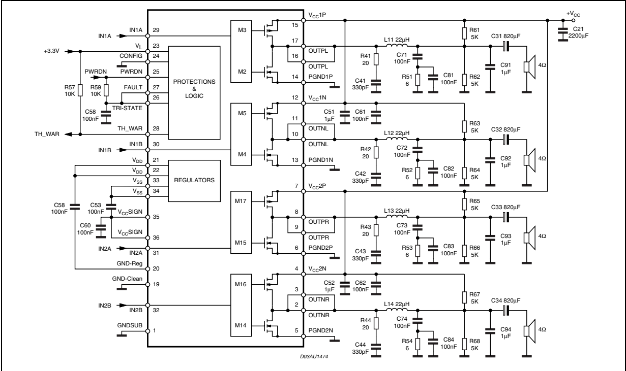
Figure 7. Typical Quad Half Bridge Configuration
