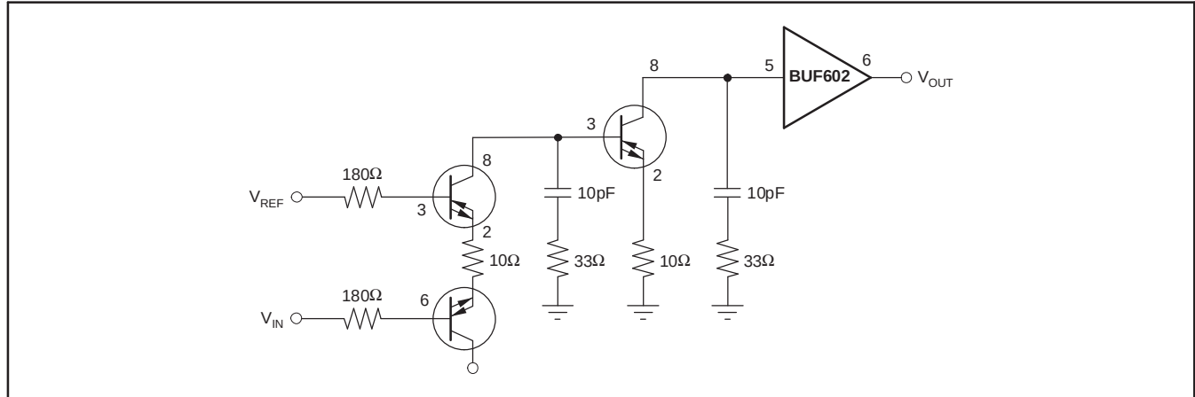
Figure 37. Control-Loop Amplifier Using Three OPA861s
