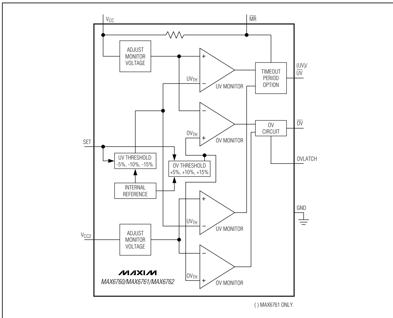
Figure 3. MAX6760/MAX6761/MAX6762 Functional Diagram
