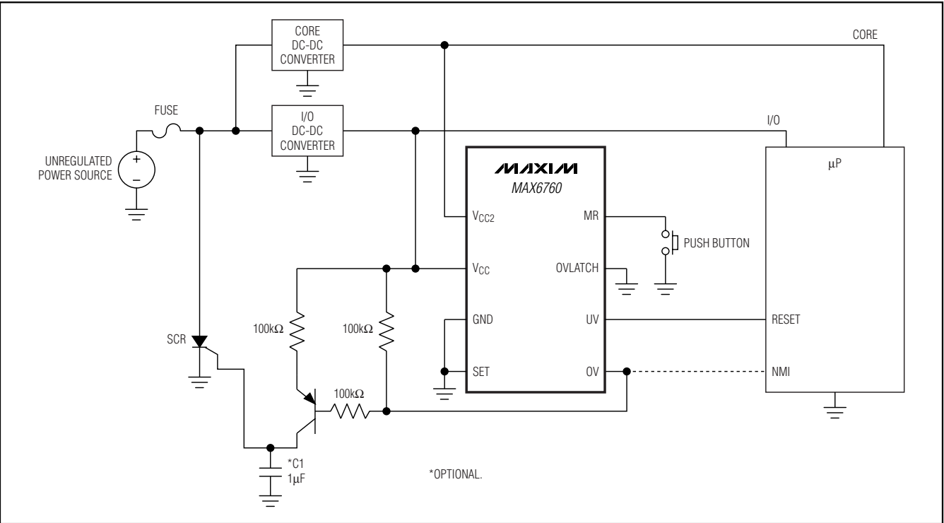
Figure 8. Microprocessor Monitoring
