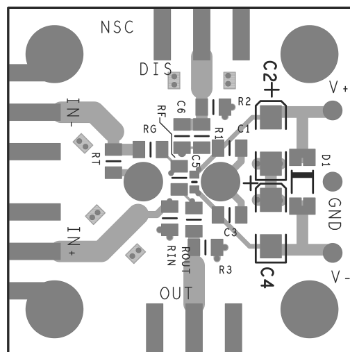
National Semiconductor Layer2 Silk NATIONAL SEMICONDUCTOR LAYER2 SILK
