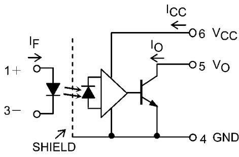
Fig. 5.1 Internal Circuit
