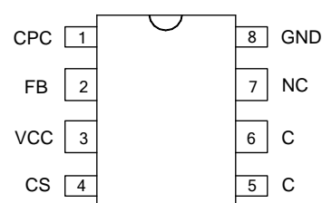
PDIP-8 (P Package) For AP3970
