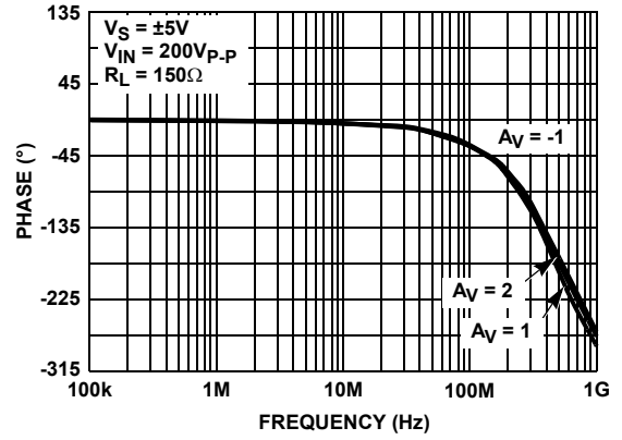
FIGURE 2. PHASE RESPONSE
