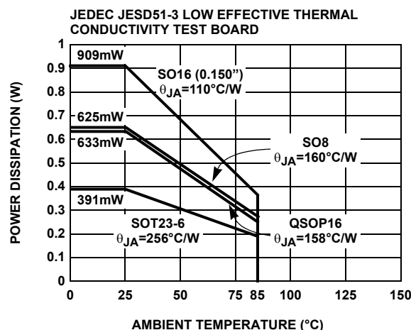
FIGURE 19. PACKAGE POWER DISSIPATION vs AMBIENT TEMPERATURE
