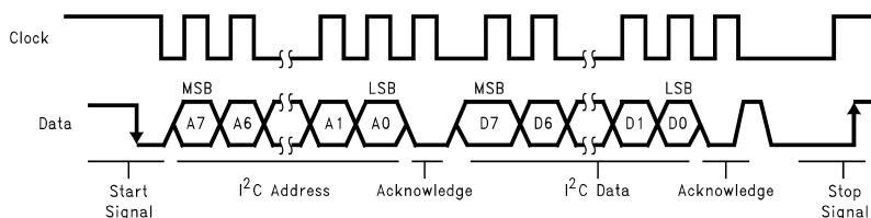
Figure 53. I 2 C Bus Format
