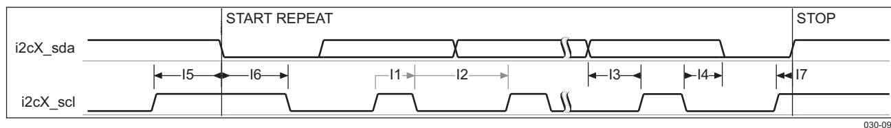
Figure 6-54. I 2 C – High-Speed Mode (1)(2)(3)
