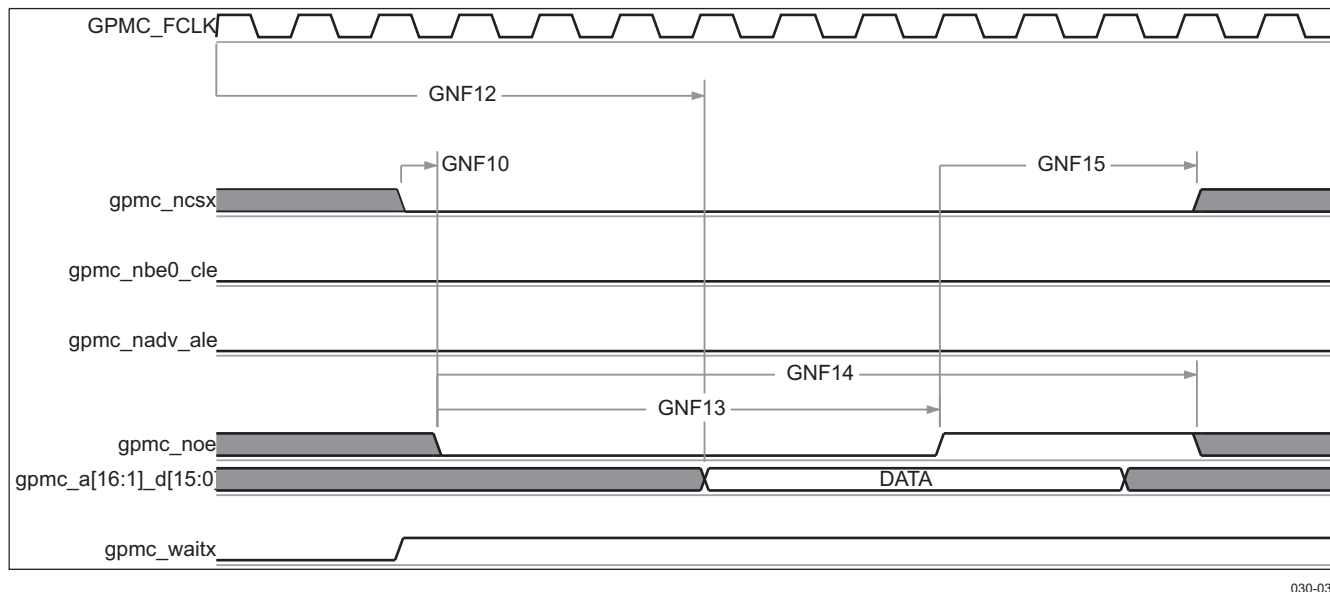
Figure 6-15. GPMC/NAND Flash – Data Read Cycle Timing (1)(2)(3)
