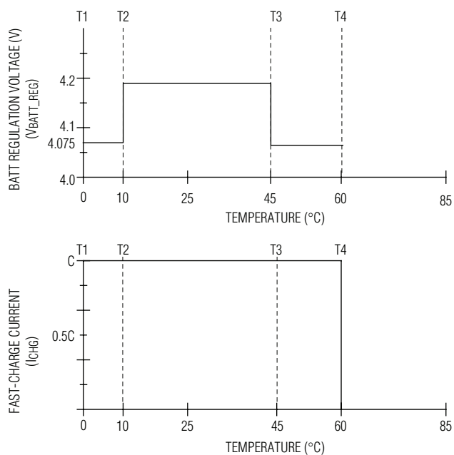
Figure 6. Safety Region 2: Fast-Charge Currents and Charge Termination Voltages
