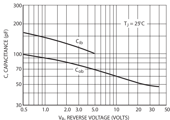
Figure 7. Capacitance
