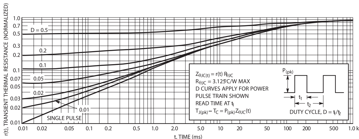
Figure 4. Thermal Response
