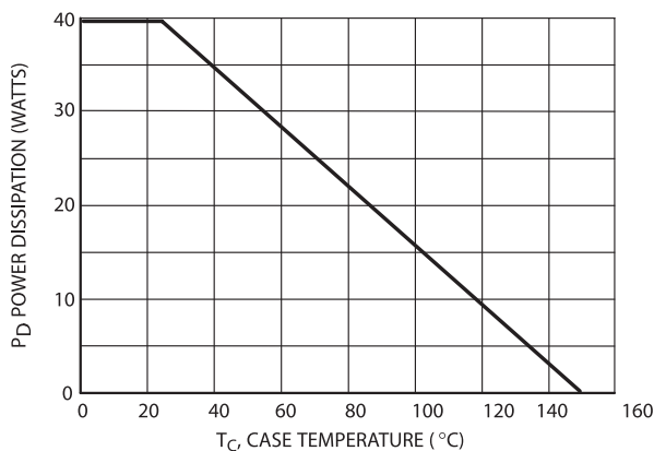
Figure 1. Power Derating
