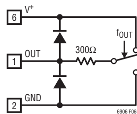
Figure 6. OUT Pin
