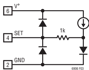
Figure 3. SET Pin
