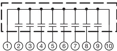
CIRCUIT CONFIGURATION "C" BOTH END LEADS GROUND
