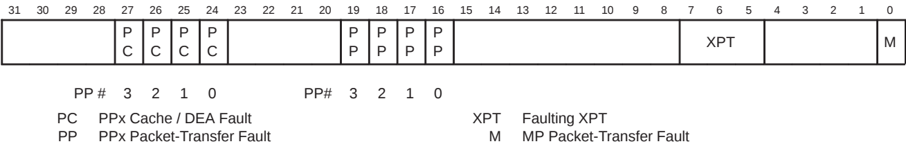
Figure 56. FLTSTS Register
