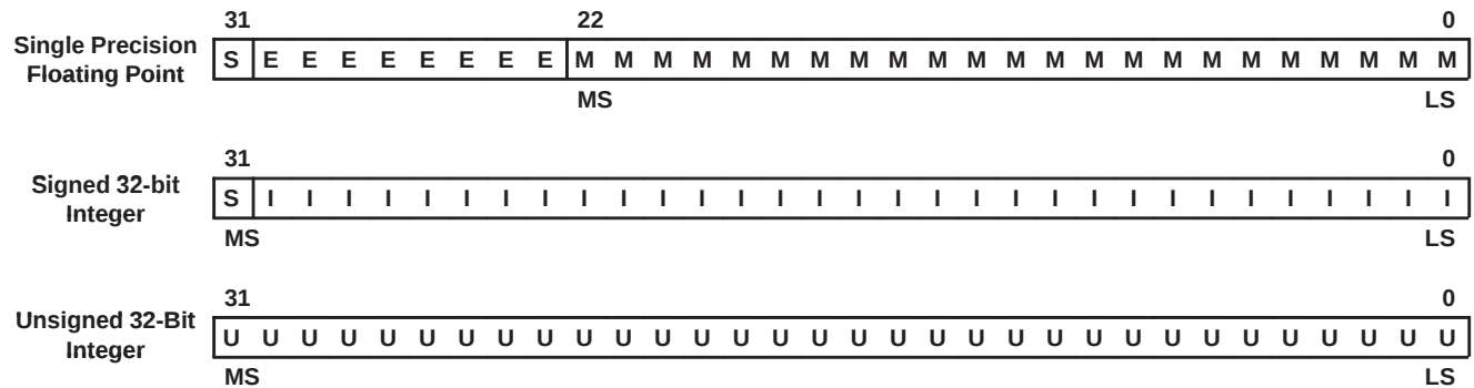
The 32-bit registers can contain signed-integer, unsigned-integer, or single precision floating-point values. Signed and unsigned bytes and halfwords are sign extended or zero-filled. Doublewords may be stored in a 64-bit even/odd register pair. Double-precision floating-point values are referenced using the even register number or the register pair. Figure 5 through Figure 7 show the register data formats.
