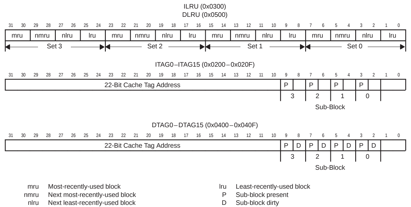
Figure 17. Cache Registers
