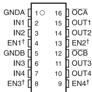
TPS2085, TPS2086 AND TPS2087 D PACKAGE
