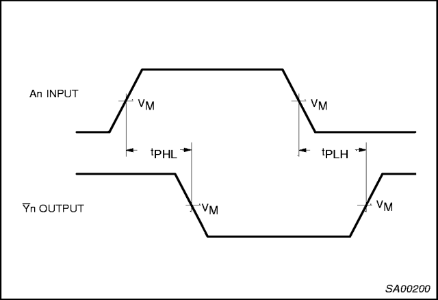
Waveform 1. Waveforms Showing the Input (An) to Output ( \bar{Y}_n ) Propagation Delays
