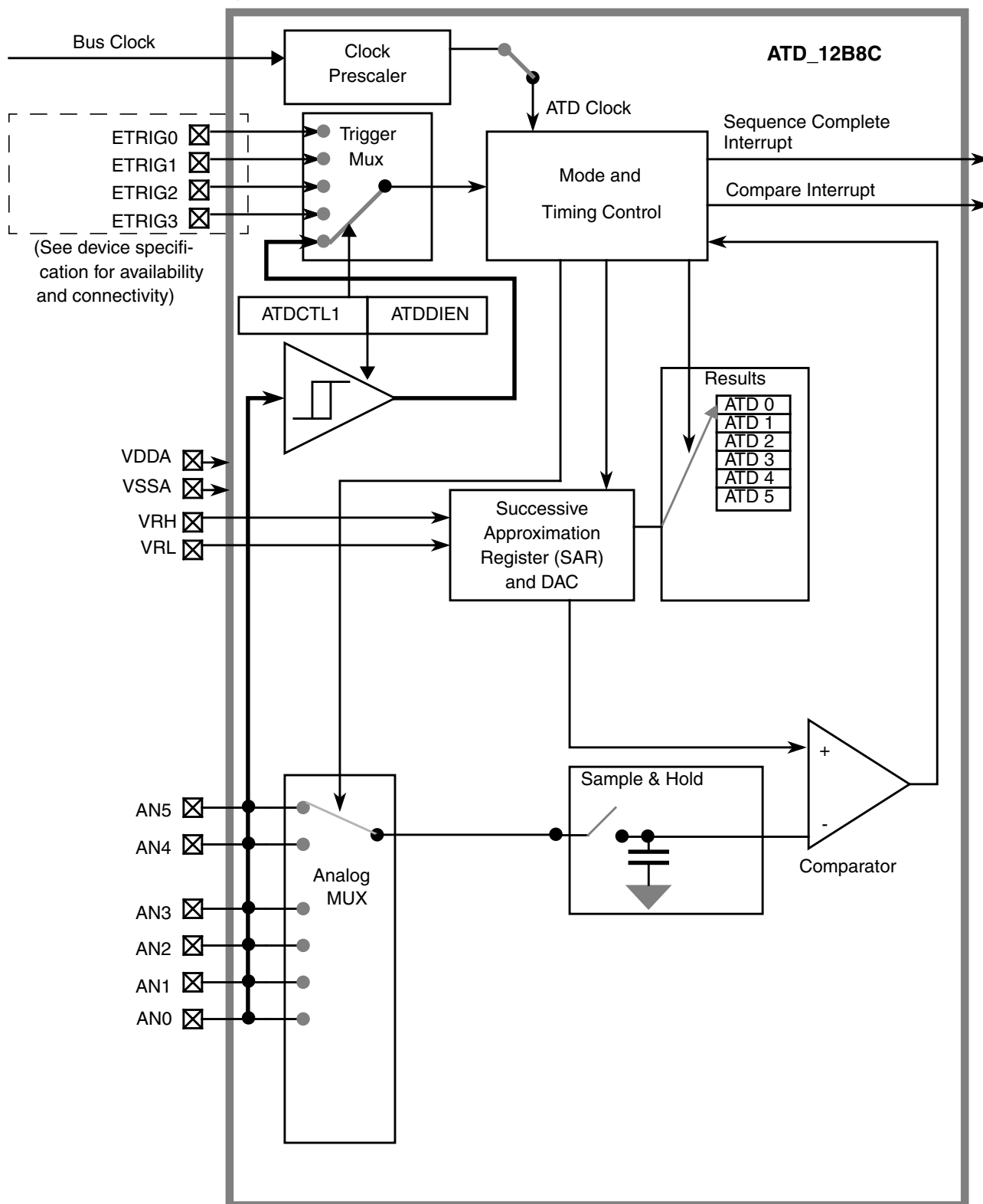
Figure 8-1. ADC12B6C Block Diagram
