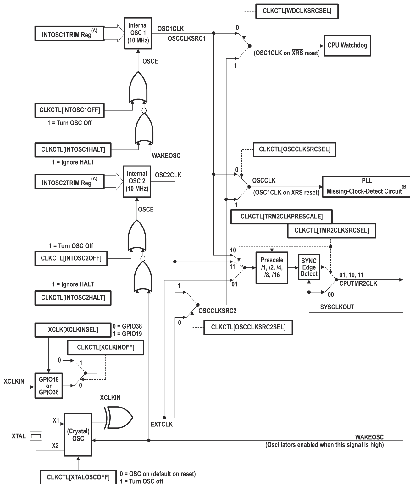
Figure 8-7. Clock Tree
