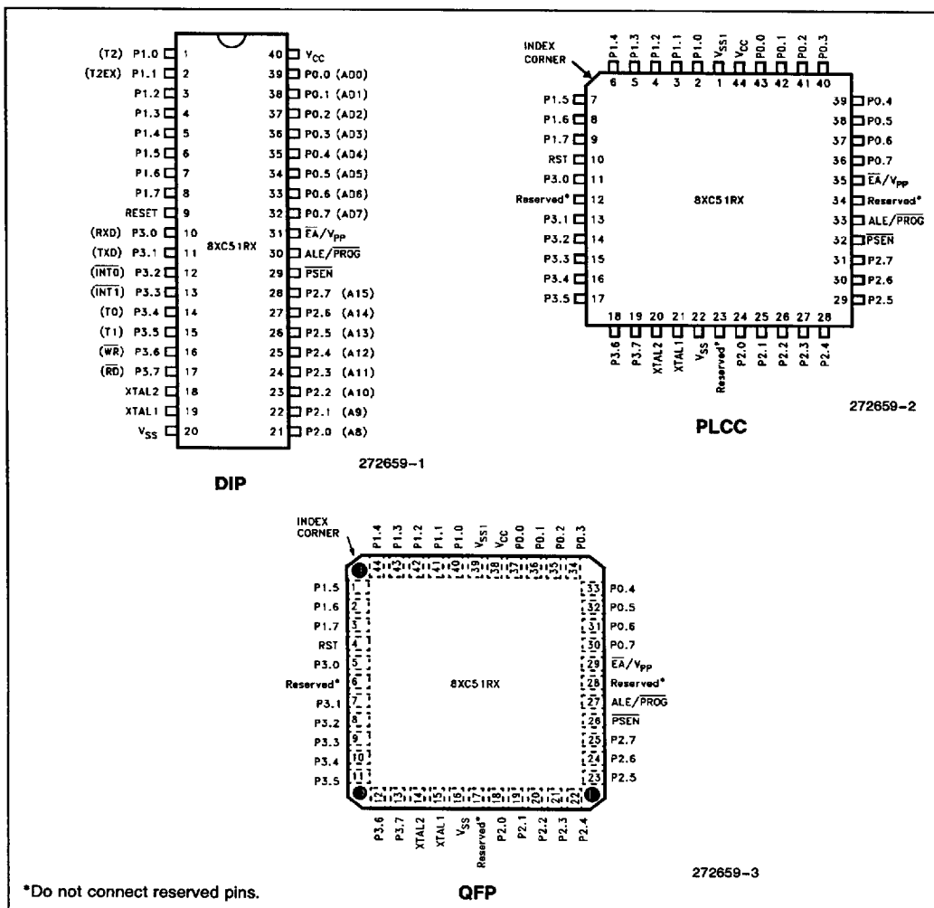
Figure 2. Pin Connections
