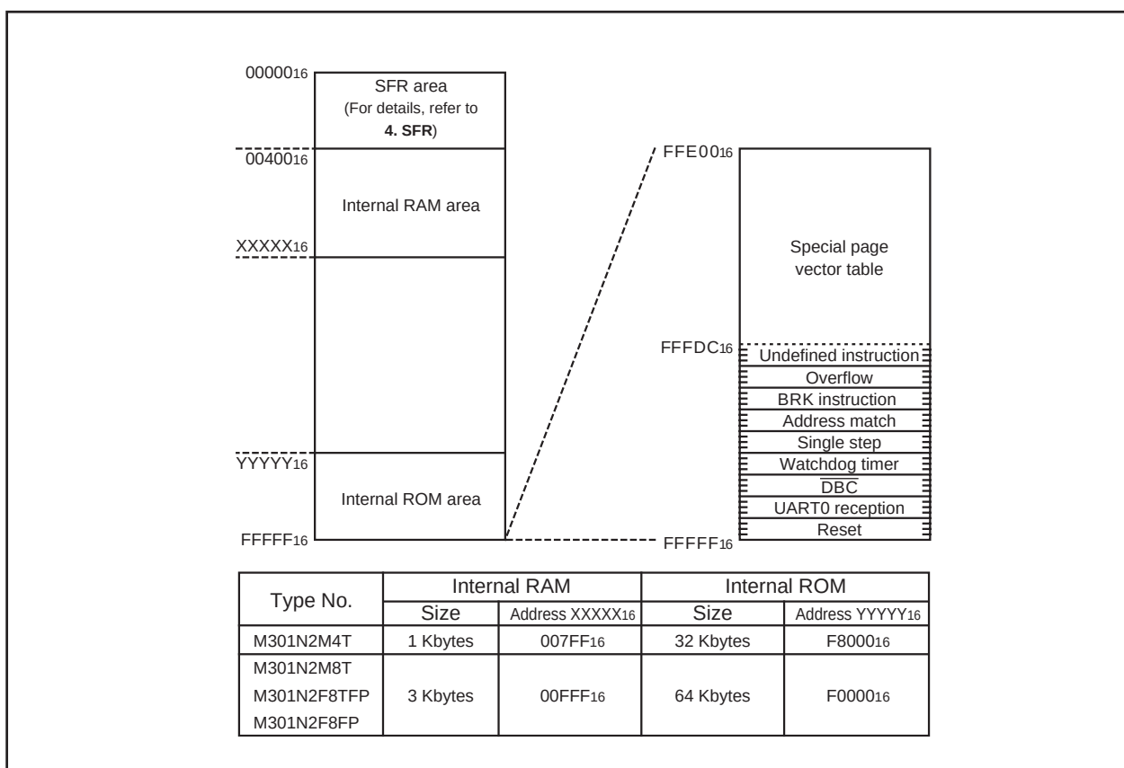
Figure 3.1 Memory map
