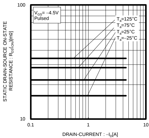
Fig.5 Static Drain-Source On-State Resistance vs. Drain Current(II)
