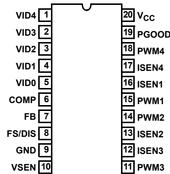
HIP6301 (SOIC) TOP VIEW
