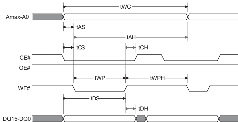
Figure 15.5 Back to Back Write Operation Timing Diagram
